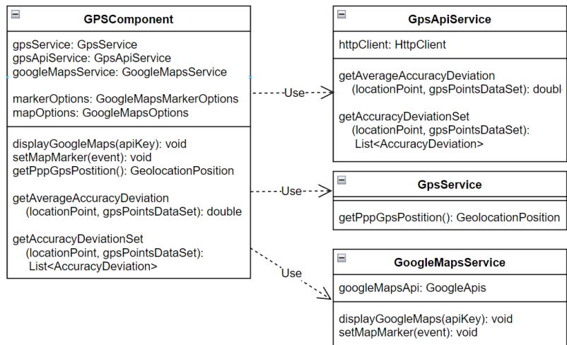
Fig. 3. Class diagram of the client side
