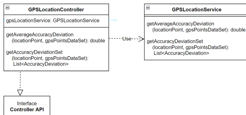
Fig. 2. Class diagram of the back end
