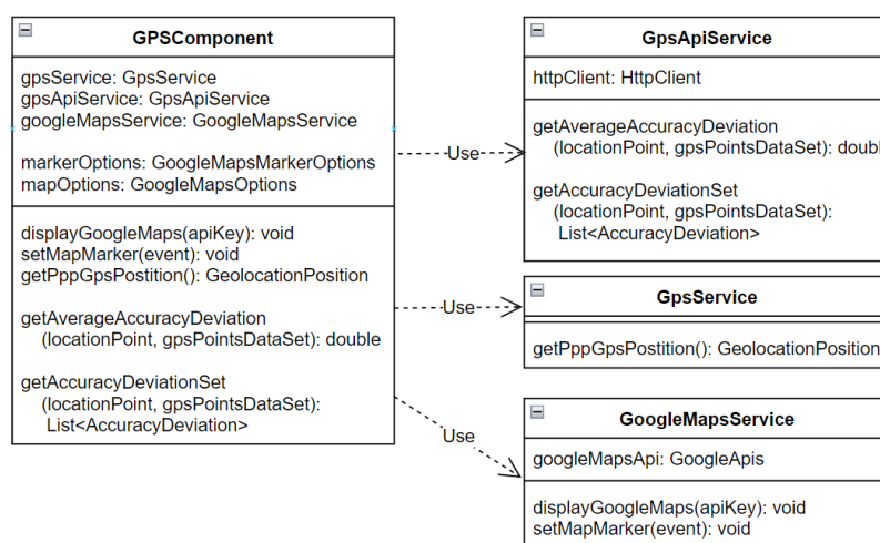
Fig. 3. Class diagram of the client side
