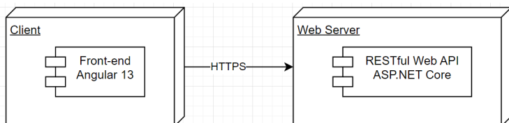
Fig. 4. Deployment diagram
