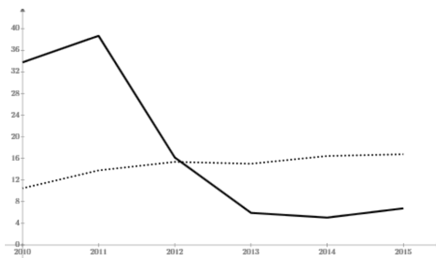
Figure 3. Actual investments (solid curve) and information about investments collected by Rosstat (point curve) at current prices; trillion P.
