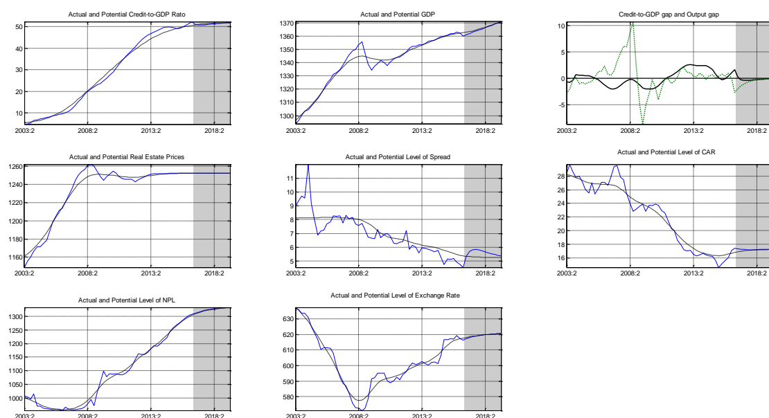
Figure 3: Model-based estimates
