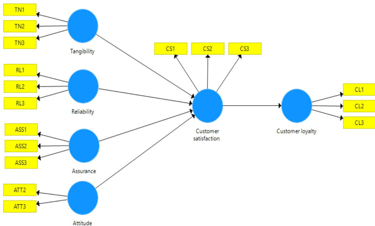
Figure 1: Theoretical Framework
