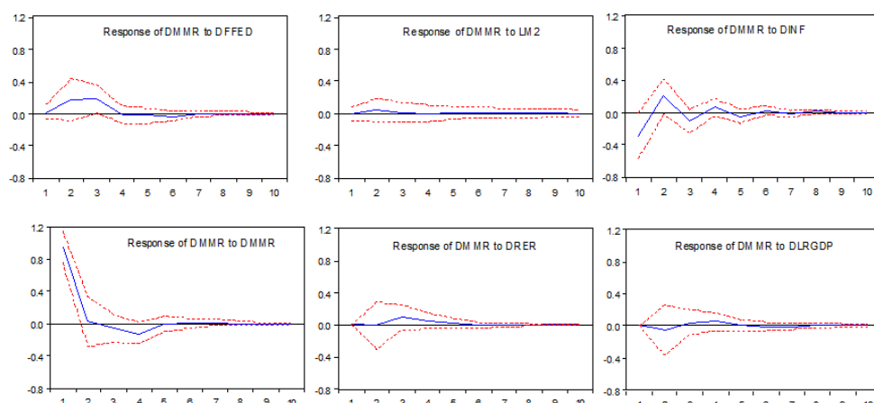
Figure 8. Impulse response functions of DMMR to structural shocks
