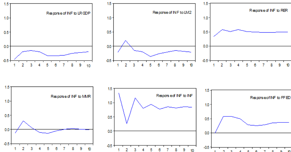
Figure 5. Response functions of INF
