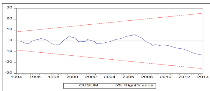
Figure 1: Cumulative sum of recursive residuals
