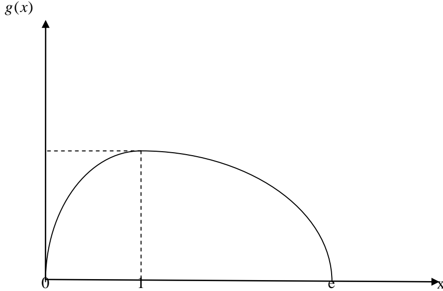
Figure 2: The shape of the Gompertz growth function g(x) = x(1 - \ln(x))
