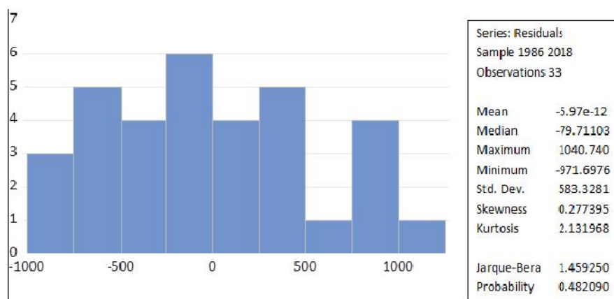
Figure 1. Normality test
