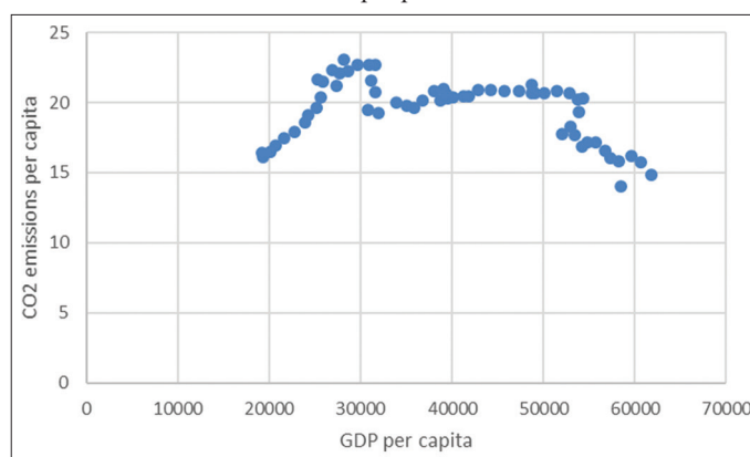
Figure 3: Scatterplot between gross domestic product per capita and tCO 2 per person
