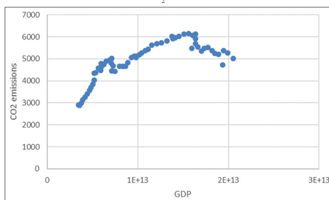
Figure 2: Scatterplot between gross domestic product and CO 2 emissions
