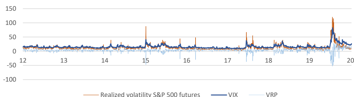
Figure 1. The volatility risk premium existence.
