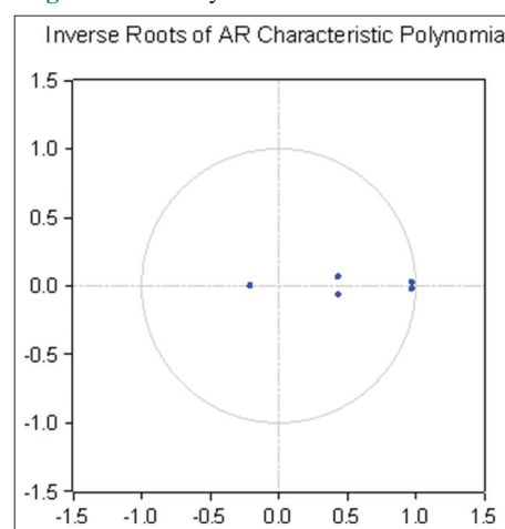
Figure 7: Stability test results for VAR model
