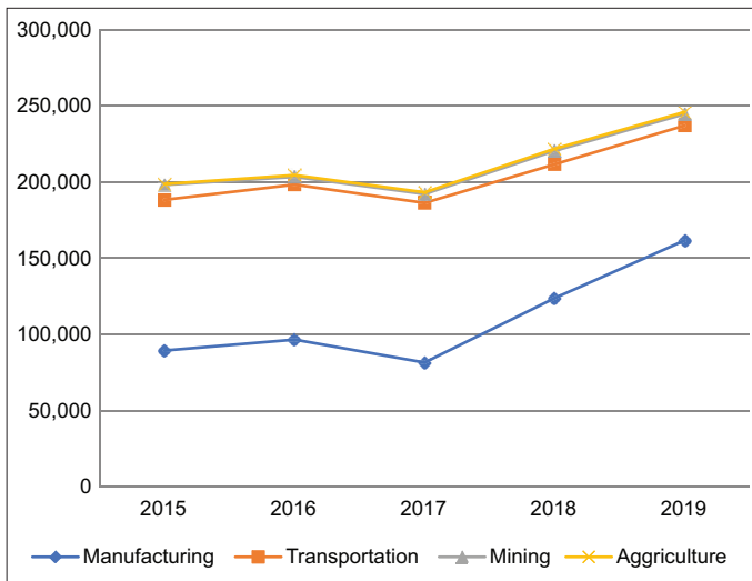
Figure 4: CO 2 Emissions by Sector in Indonesia in 2015-2019
