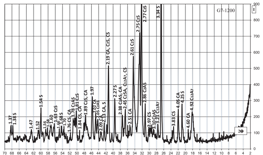
Fig. 5. X-ray diffraction of binder sample K7 after firing at 1200 °C
