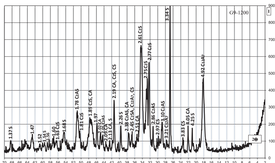
Fig. 6. X-ray diffraction of binder sample K9 after firing at 1200 °C
