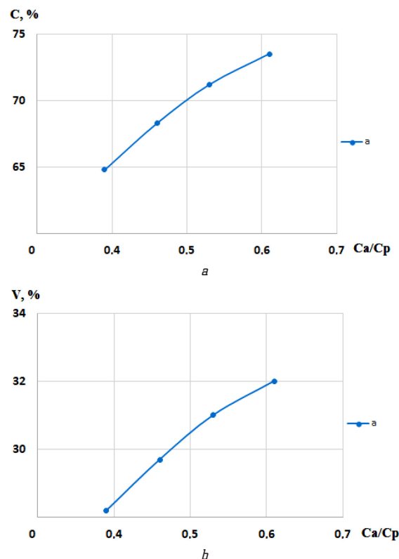
Fig. 4. Dependence of the content ( C ) of chalk ( a ) and emissions ( V ) of CO_2 ( b ) on the quantitative ratio of aluminium hydroxide and pyloquartz ( Ca/Cp )
