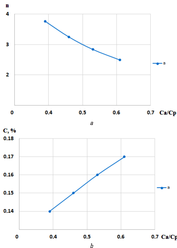
Fig. 3. Dependence of the silica modulus ( n ) of the binder ( a ) and of the content ( C ) of colored oxides ( b ) from the quantitative ratio of hydrate of aluminium oxide and pyloquartz ( Ca/Cp ) in the chalk-based system
