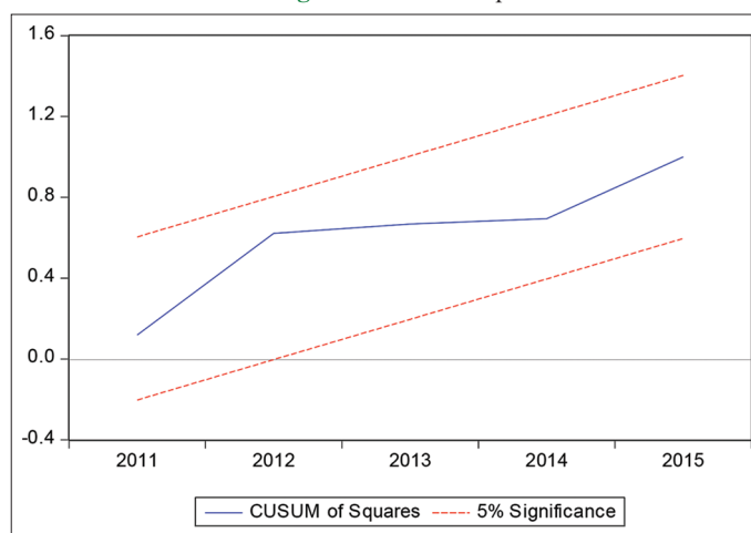
Figure 3: CUSUMsq
