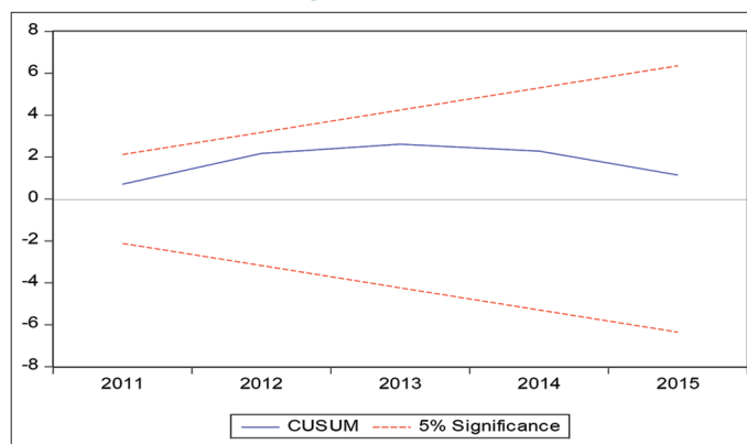
Figure 2: CUSUM
