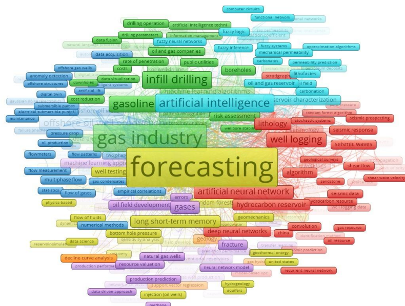
Figure 2: Word cloud
