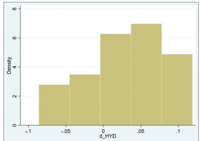
Figure 3: Distribution of pointwise marginal effect
