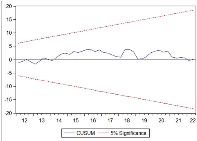
Figure 1: CUSUM for model 1
