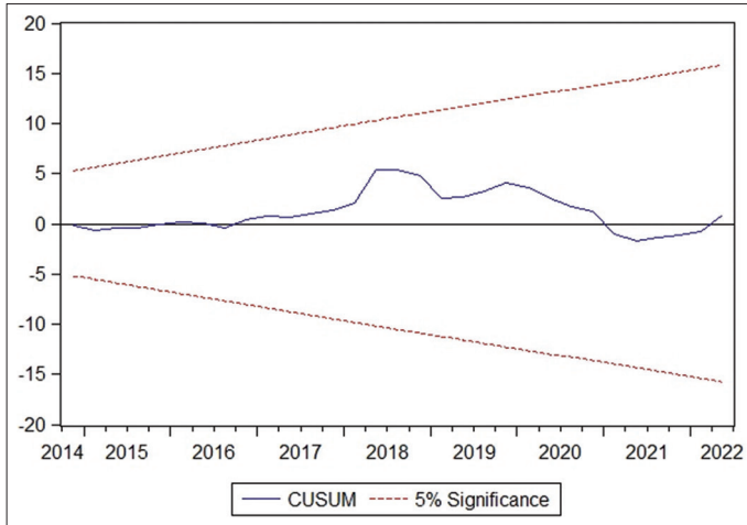
Figure 2: CUSUM for model 2
