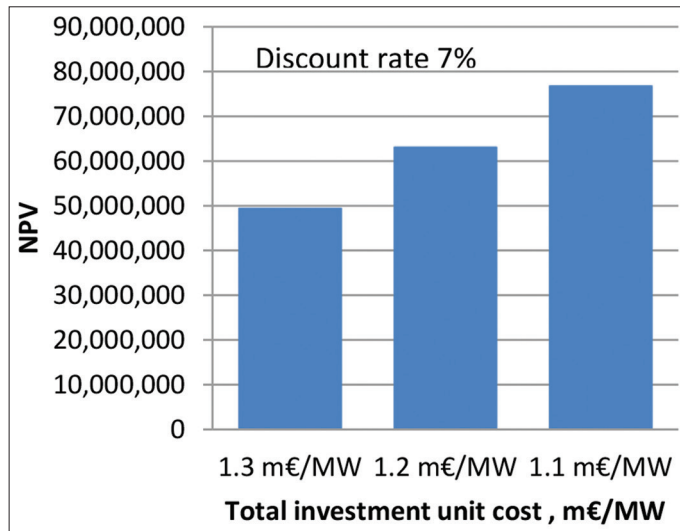
Figure 18: Graphical representation NPV = f(\text{total unit cost of installation; } r = 7\%)
