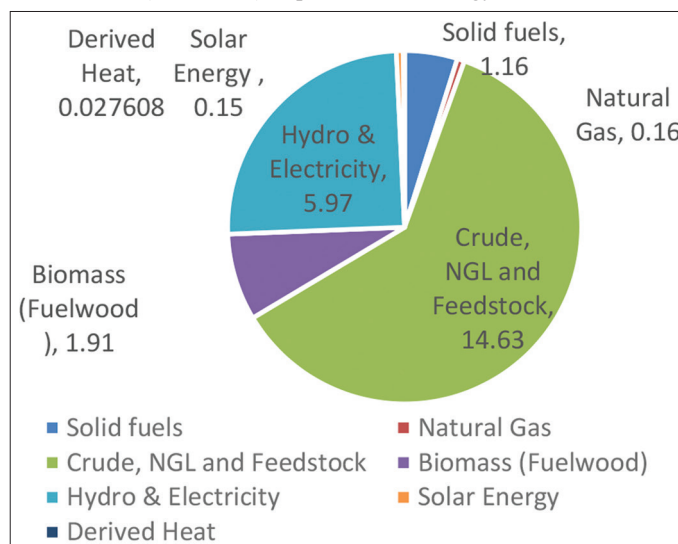
Figure 28: Annual energy consumption by fuel type in Albania (TWh) (ERE, 2018): Input values in EnergyPLAN
