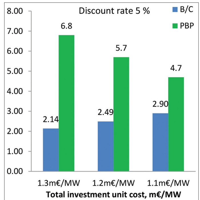
Figure 22: Graphical layout [B/C and PBP] = f (total unit cost of installation; r = 5%)
