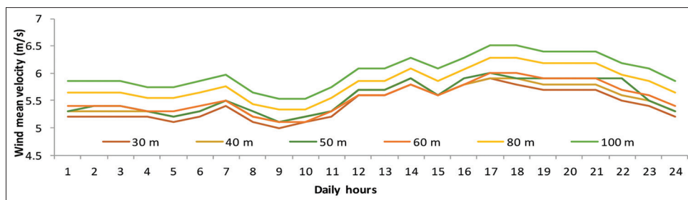
Figure 8: Daily variation of mean wind speed (m/s) measured at altitudes of 30, 40, 50, 60, 80 and 100 m, Verniku, Period 24.02.2008-5.02.2009 (ERE, 2018)
