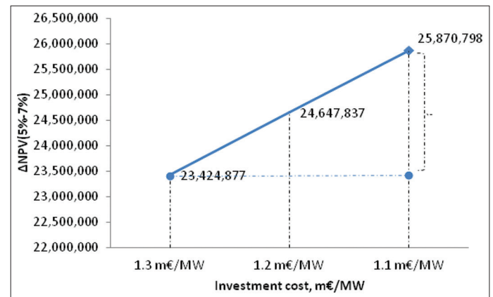
Figure 20: Graphical representation \Delta NPV = f(\text{total unit cost of installation; } \Delta r = 5-7\%)
