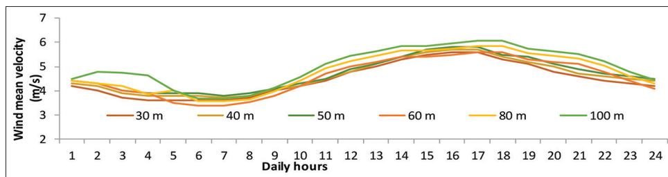
Figure 7: Daily variation of mean wind speed (m/s) measured at altitudes of 30, 40, 50, 60, 80 and 100 m, Nizhaveci, Period 24.02.2008-5.02.2009 (ERE, 2018)
