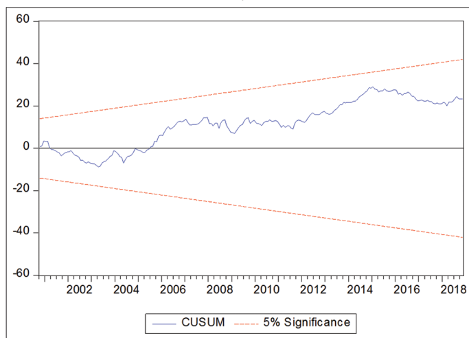
Figure 2: Plots of cumulative sum (CUSUM) statistics for coefficients stability tests
