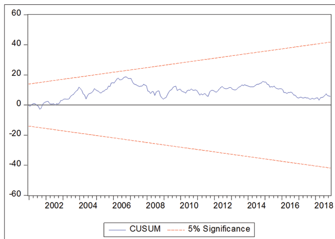
Figure 1: Plots of cumulative sum statistics for coefficients stability tests
