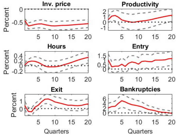
(b) Investment-specific shocks
